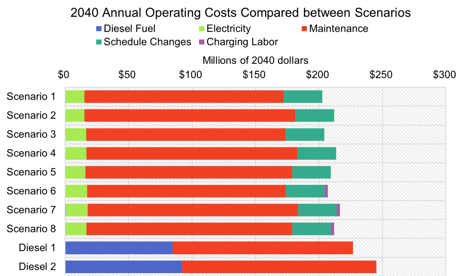
Figure 15 – 2040 Operating costs compared between scenarios Note that diesel fuel costs for heaters on electric buses are included, but the bar is very small.
